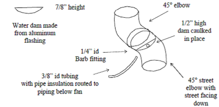
Figure 5 - Dilts Drain schematic
